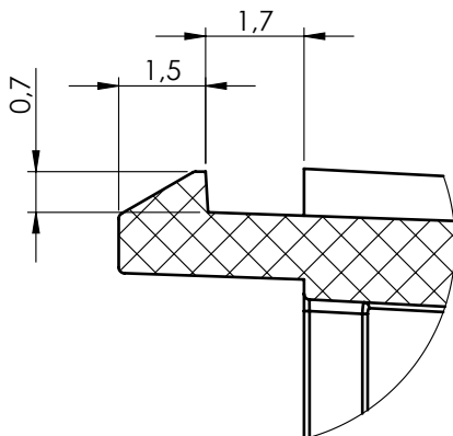
DETAIL C SCALE 7 : 1
