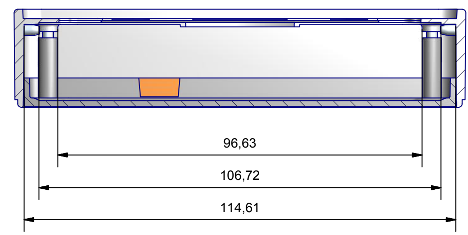
B-B (1:1)
